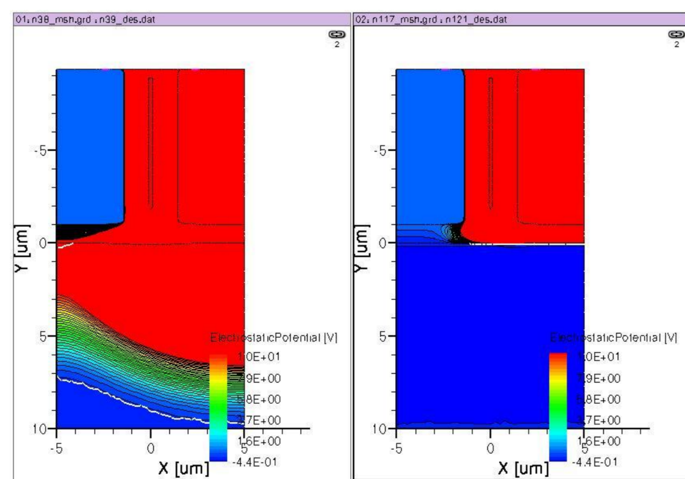
Trench and SOI optimisation
